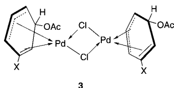
Scheme 3. Suggested dimer intermediate in the coupling of benzene with \text{NaOAc} and \text{PdCl}_2 .
